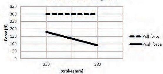
Stroke/force diagram
